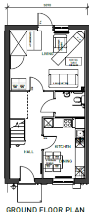
Left: Front elevation drawing 2bed affordable house Above: Floor plans for 2bed affordable house
