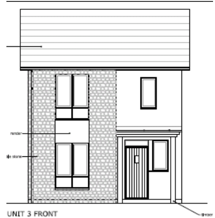
Left: Artists impression from main road Above: Elevation drawing of 3 bed house
