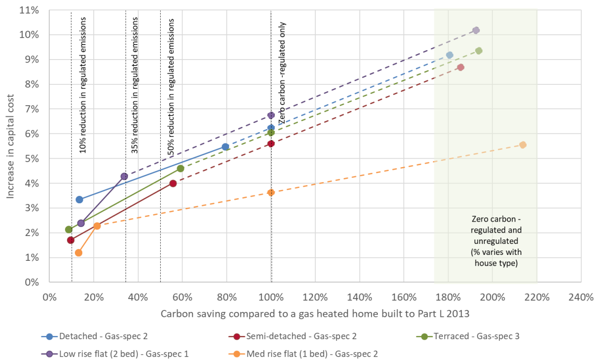
Figure 4.4 Cost and performance of options to achieve policy option 2 with gas heating
