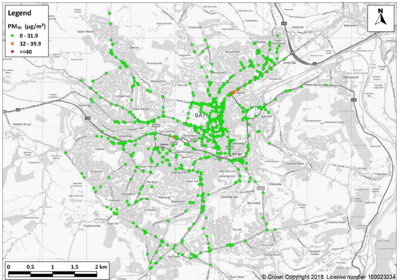
Figure 7: Predicted PM 10 concentrations in 2017 at receptor locations relevant to the national air quality objective (annual mean)
