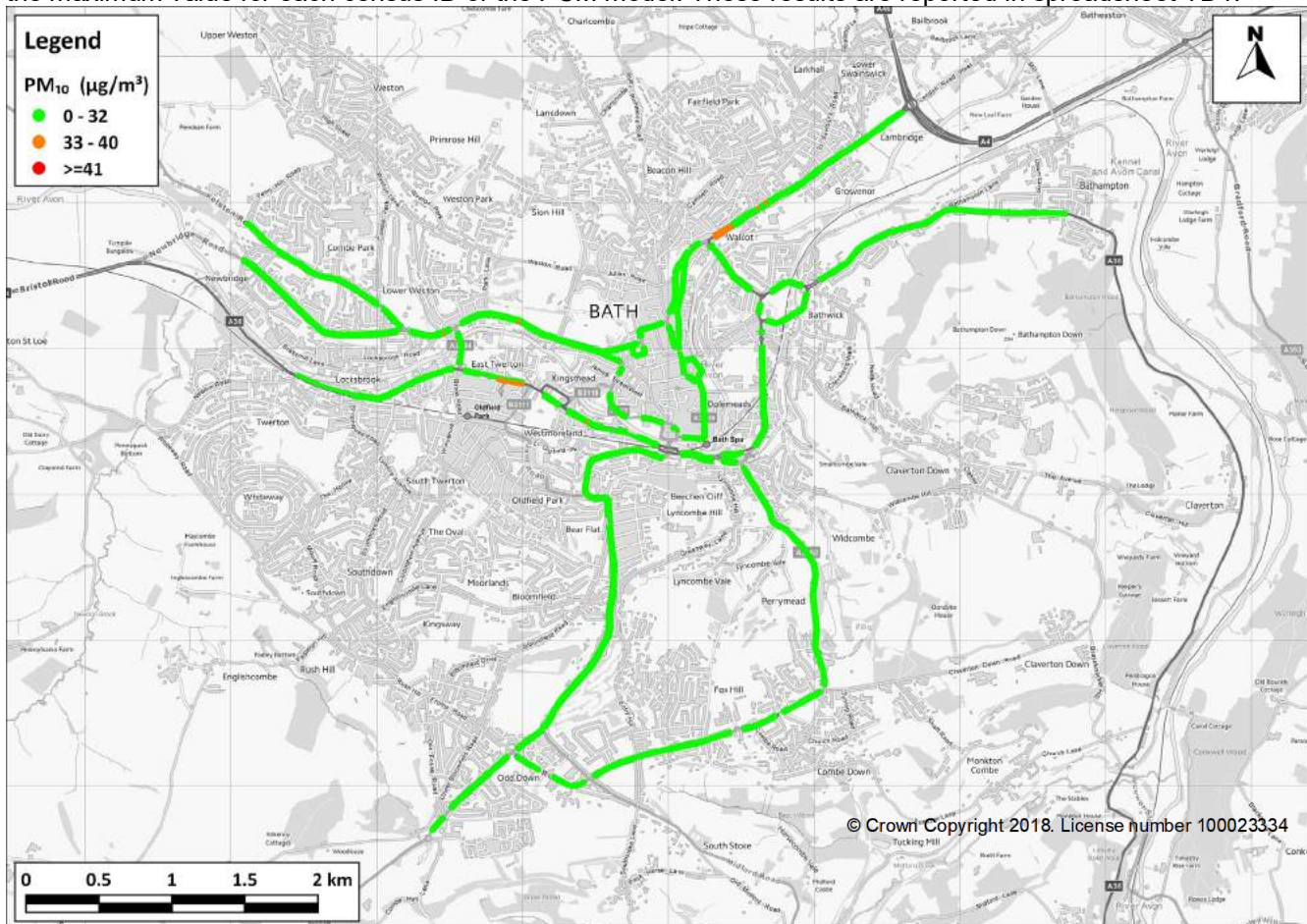
Figure 11: Predicted PM 10 concentrations in 2017 at PCM-equivalent receptor locations
