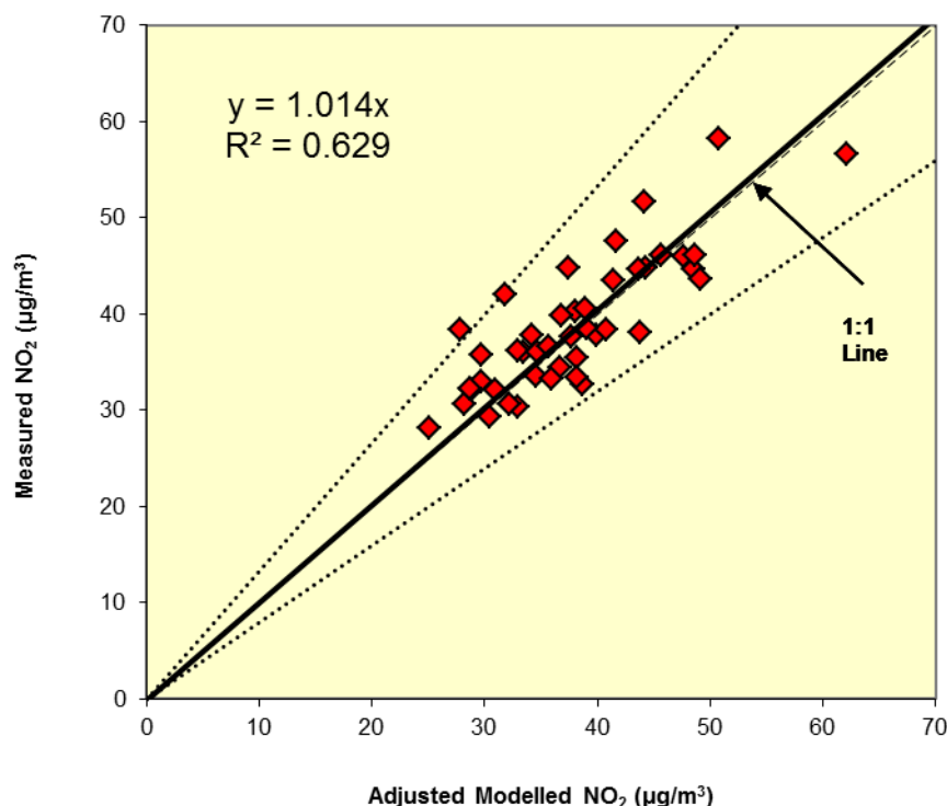
Figure 2: Comparison of Measured Total NO 2 to Final Adjusted Modelled Total NO 2 Concentrations. The dashed lines show \pm 25\% .
