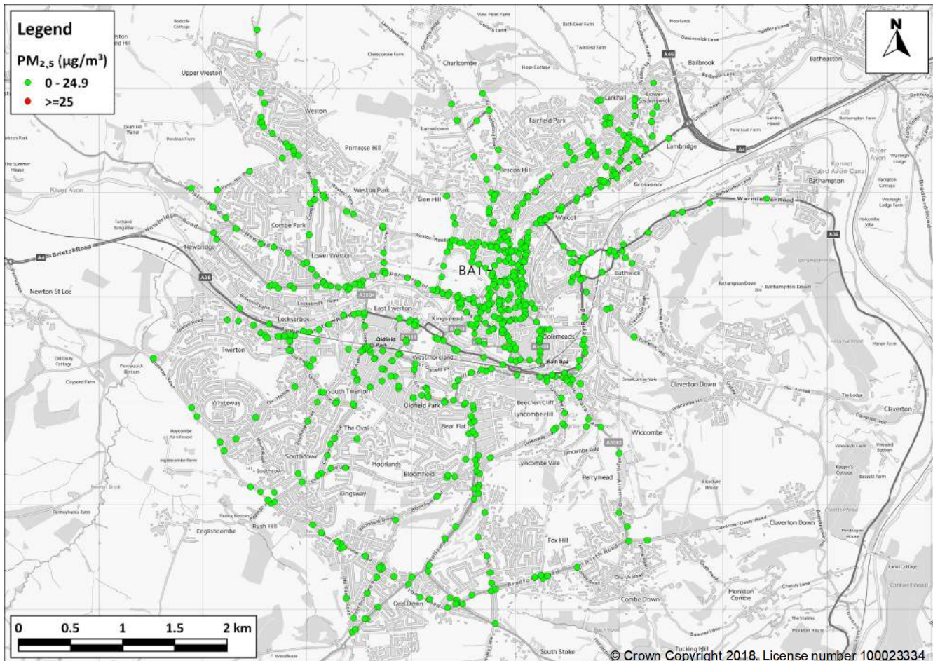
Figure 10: Predicted PM 2.5 concentrations in 2021 at receptor locations relevant to the national air quality objective (annual mean)
