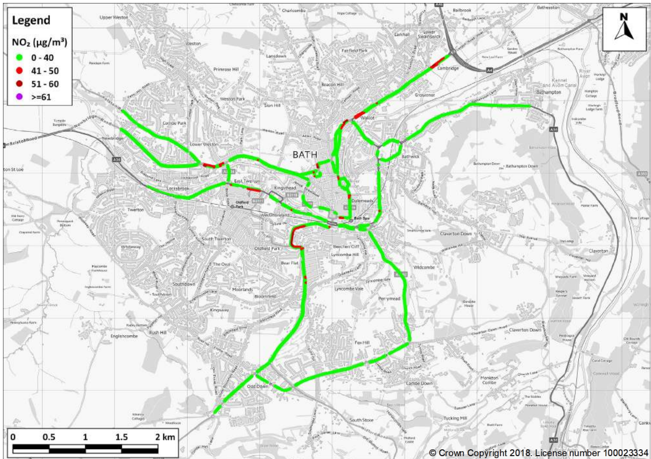
Figure 6: Predicted NO 2 concentrations in 2021 at PCM-equivalent receptor locations (annual mean)
