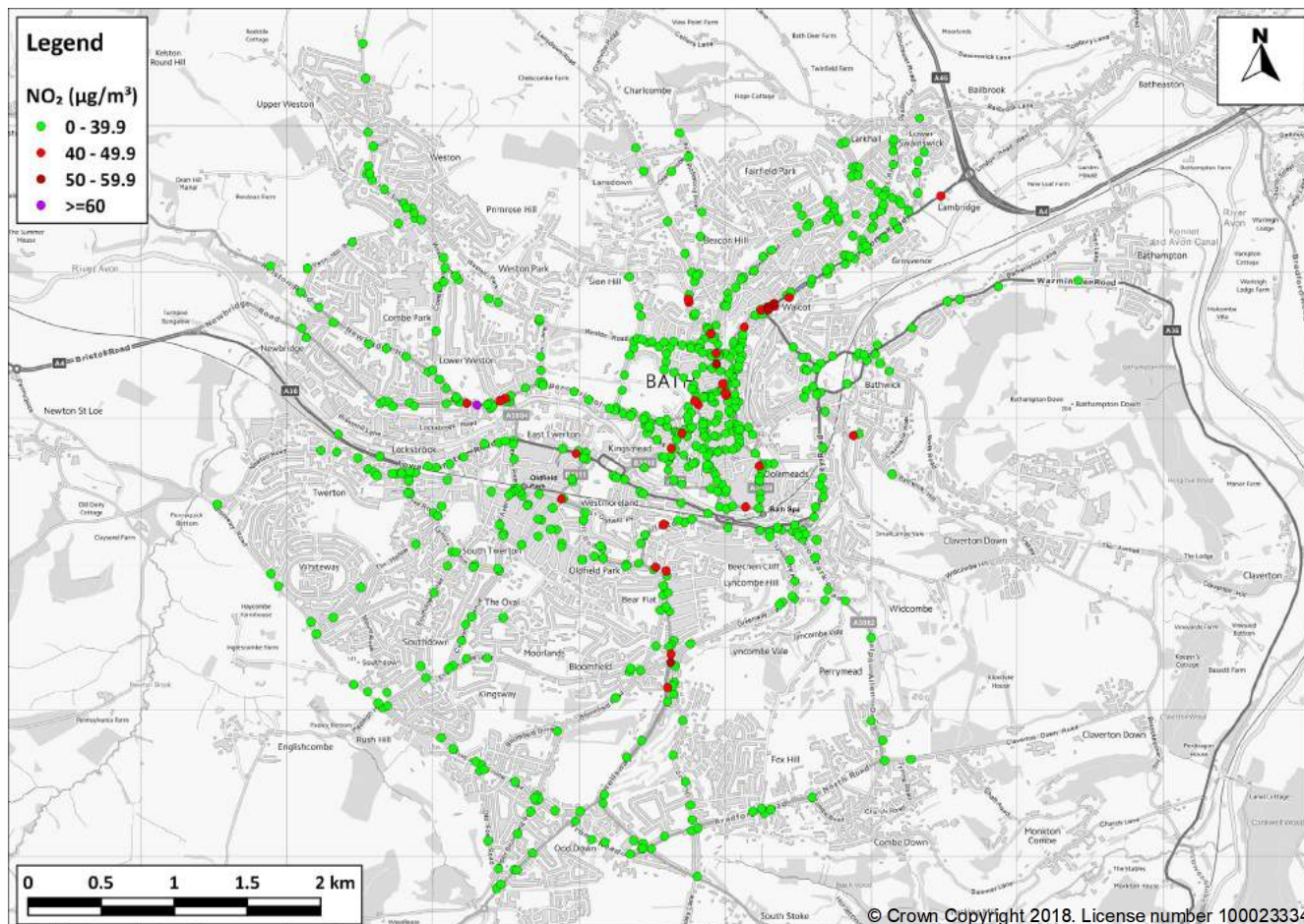
Figure 4: Predicted NO 2 concentrations in 2021 at receptor locations relevant to the national air quality objective (annual mean)
