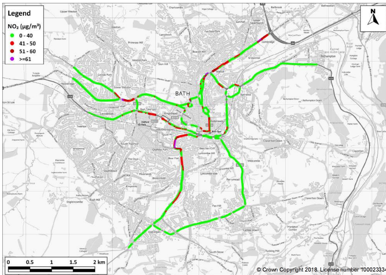
Figure 5: Predicted NO 2 concentrations in 2017 at PCM-equivalent receptor locations (annual mean)
