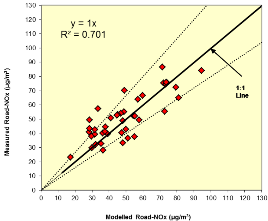
Figure 8: Comparison of Measured Road NO x to Modelled Road NO x Concentrations. The dashed lines show ± 25%.
