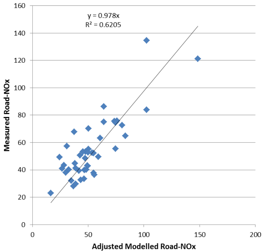
Figure 6: Comparison of Measured Road-NOx to Adjusted Modelled Road-NOx Concentrations at Gradient and Non-gradient Roads ( \mu\text{g}/\text{m}^3 )
