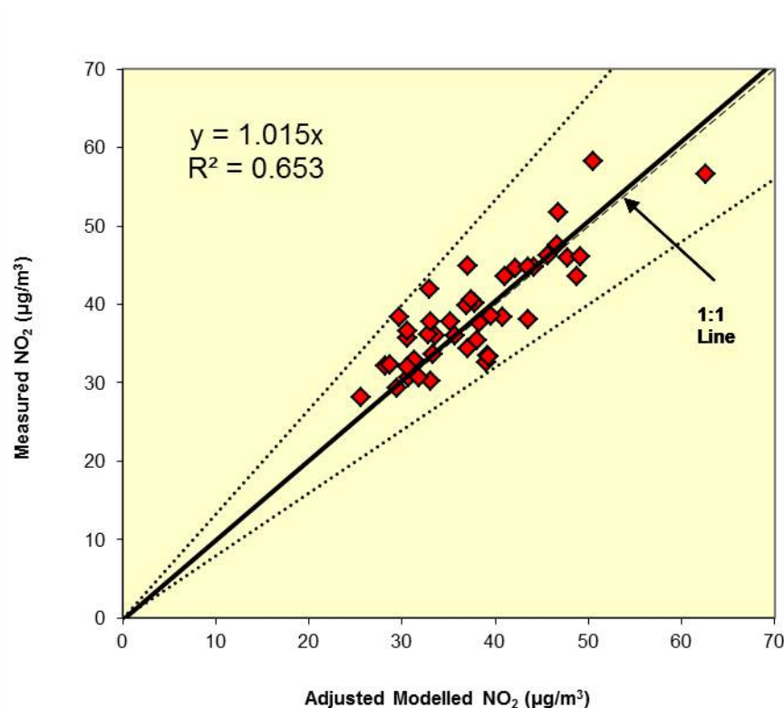
Figure 2: Comparison of Measured Total NO 2 to Final Adjusted Modelled Total NO 2 Concentrations. The dashed lines show \pm 25\% .
