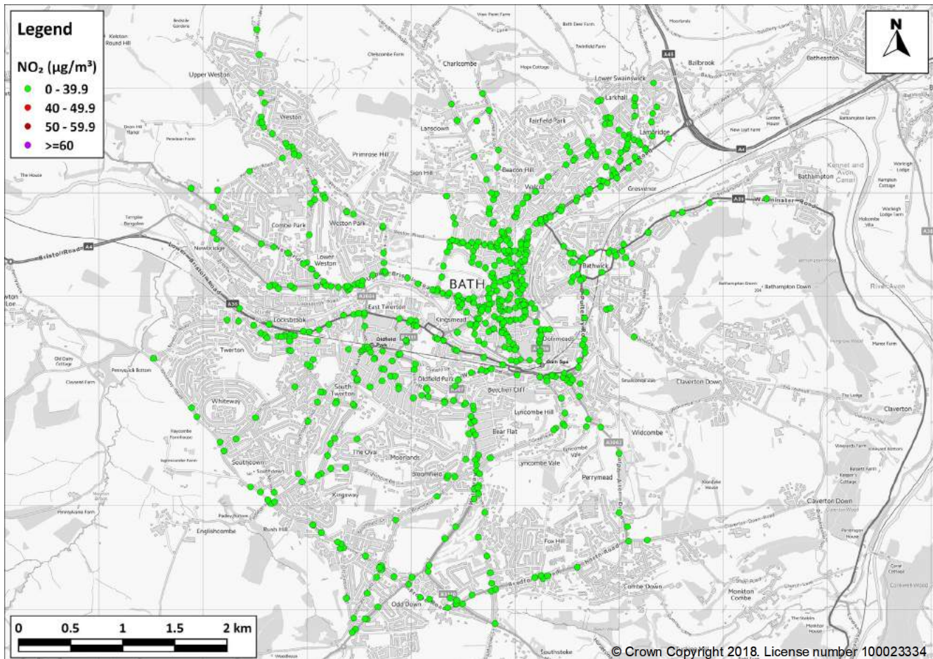
Figure 24: Predicted NO 2 concentrations in 2021 with a CAZ D (£9/£100 charge) With Traffic Management and Concessions at receptor locations relevant to the national air quality objective (annual mean)
