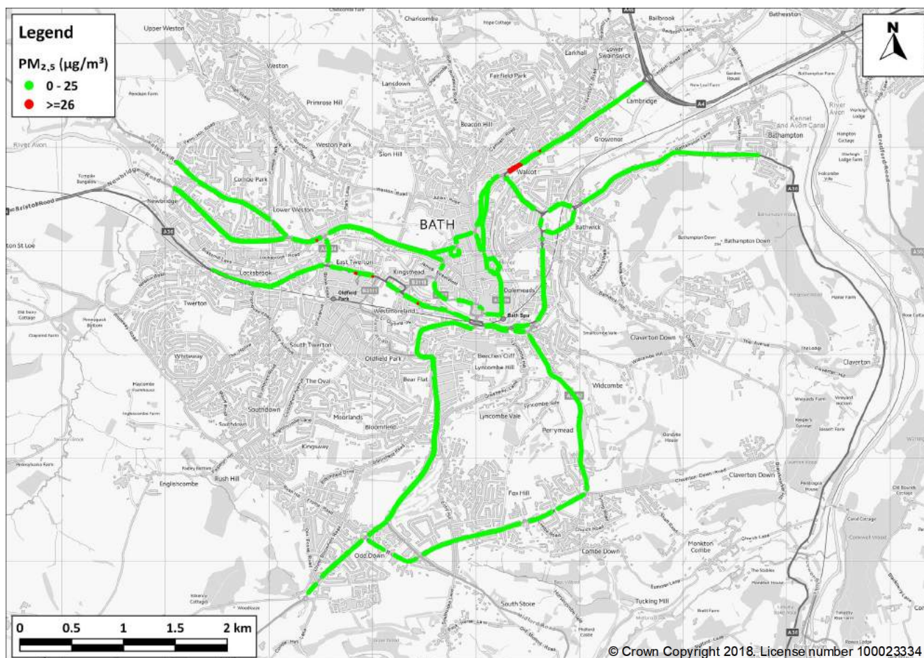
Figure 13: Predicted PM 2.5 concentrations in 2017 at PCM-equivalent receptor locations
