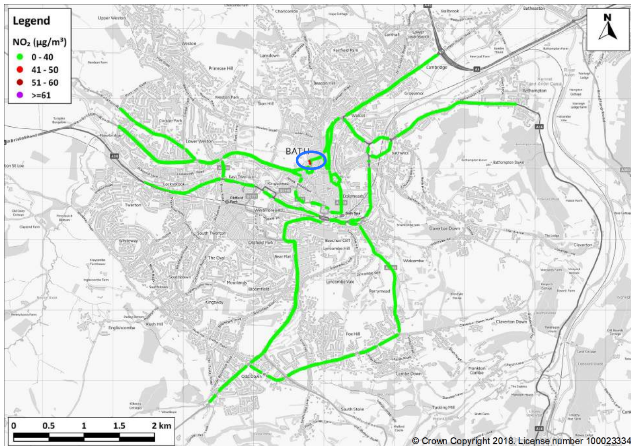
Figure 15: Predicted NO 2 concentrations in 2021 with a CAZ C (£9/£100 charge) at PCM-equivalent receptor locations (exceedance location shown within blue oval)
