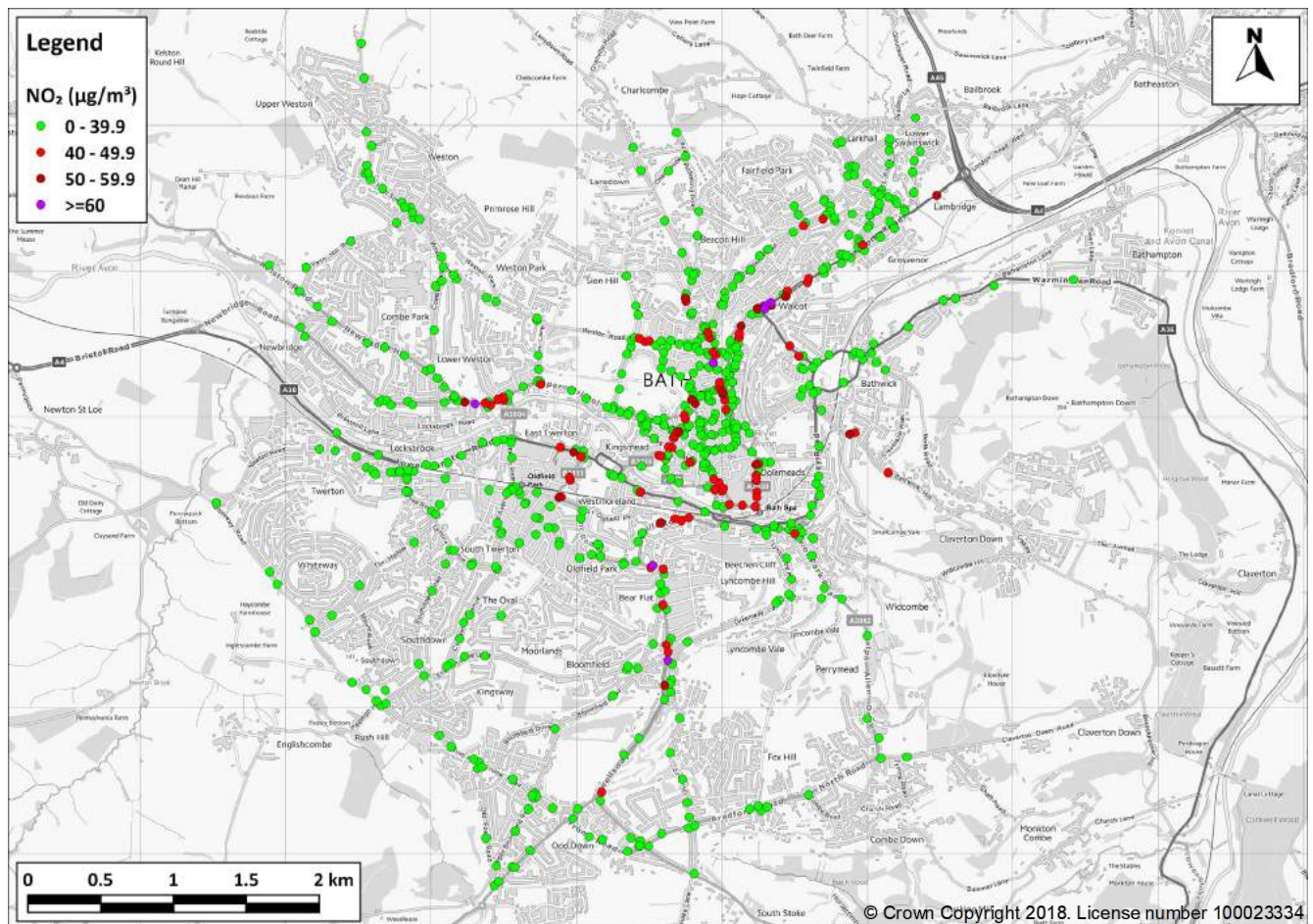
Figure 3: Predicted NO 2 concentrations in 2017 at receptor locations relevant to the national air quality objective (annual mean)
