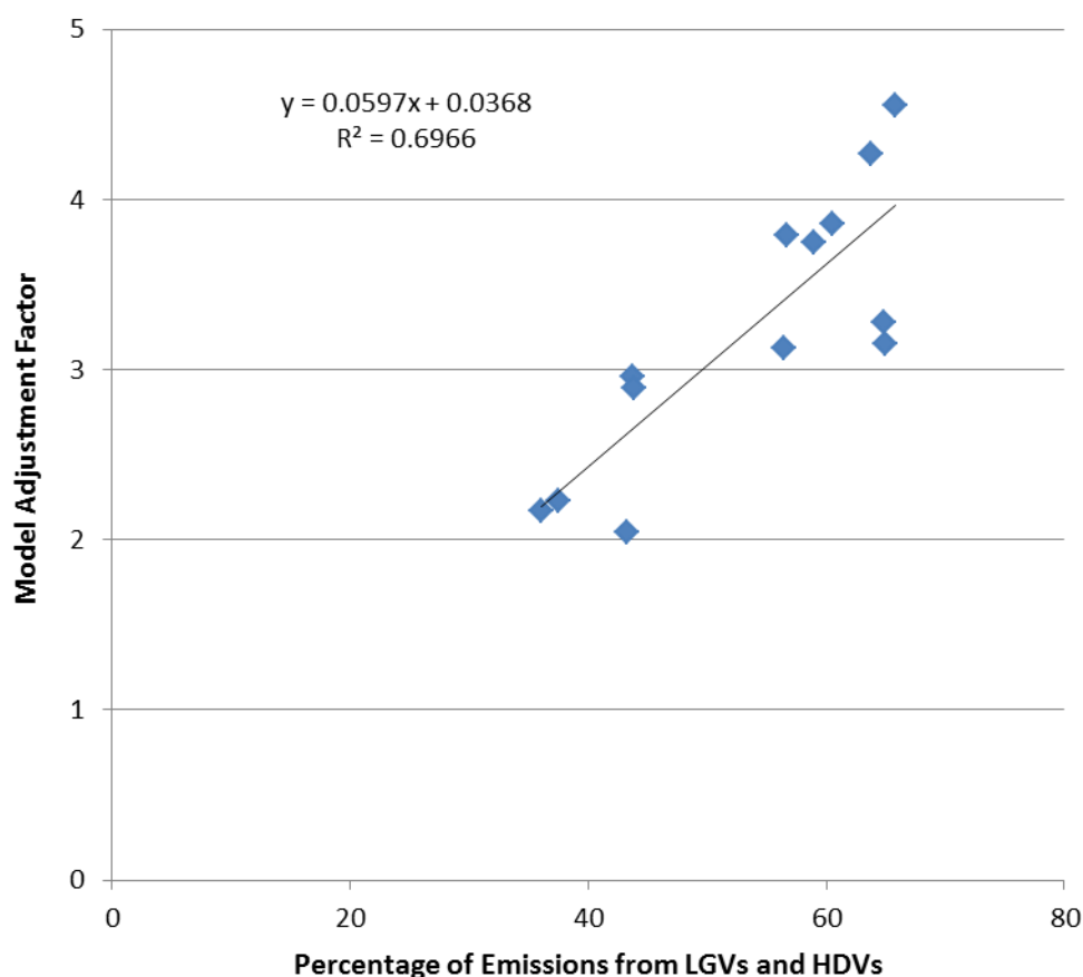
Figure 3: Measured Road-NO x divided by Modelled Road-NO x on Gradient Roads (Y Axis) vs Percentage of NO x Emissions from the Nearest Road which are Assumed to Come from LGVs and HDVs (X Axis)
