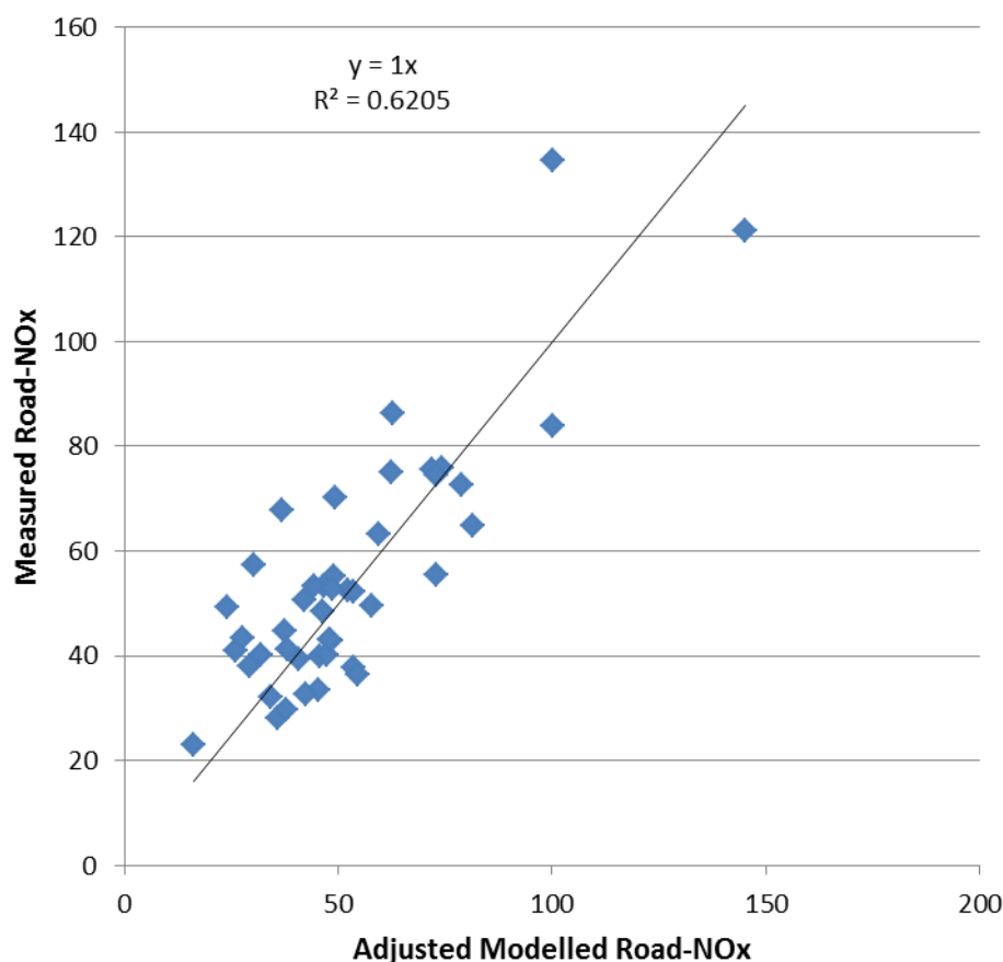
Figure 7: Comparison of Measured Road-NOx to Adjusted Modelled Road-NOx Concentrations at Gradient and Non-gradient Roads after Iterating ( \mu\text{g}/\text{m}^3 )
