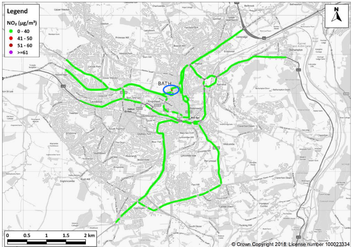
Figure 17: Predicted NO 2 concentrations in 2021 with a CAZ D (£7.50/£100 charge) at PCM-equivalent receptors (exceedance location shown within blue oval)
