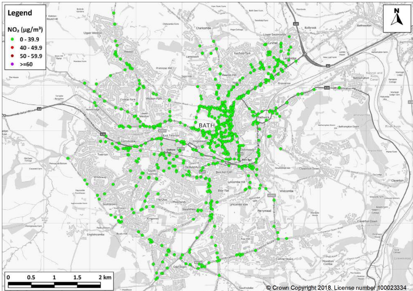
Figure 18: Predicted NO 2 concentrations in 2021 with a CAZ D (£7.50/£100 charge) at receptor locations relevant to the national air quality objective (annual mean)
