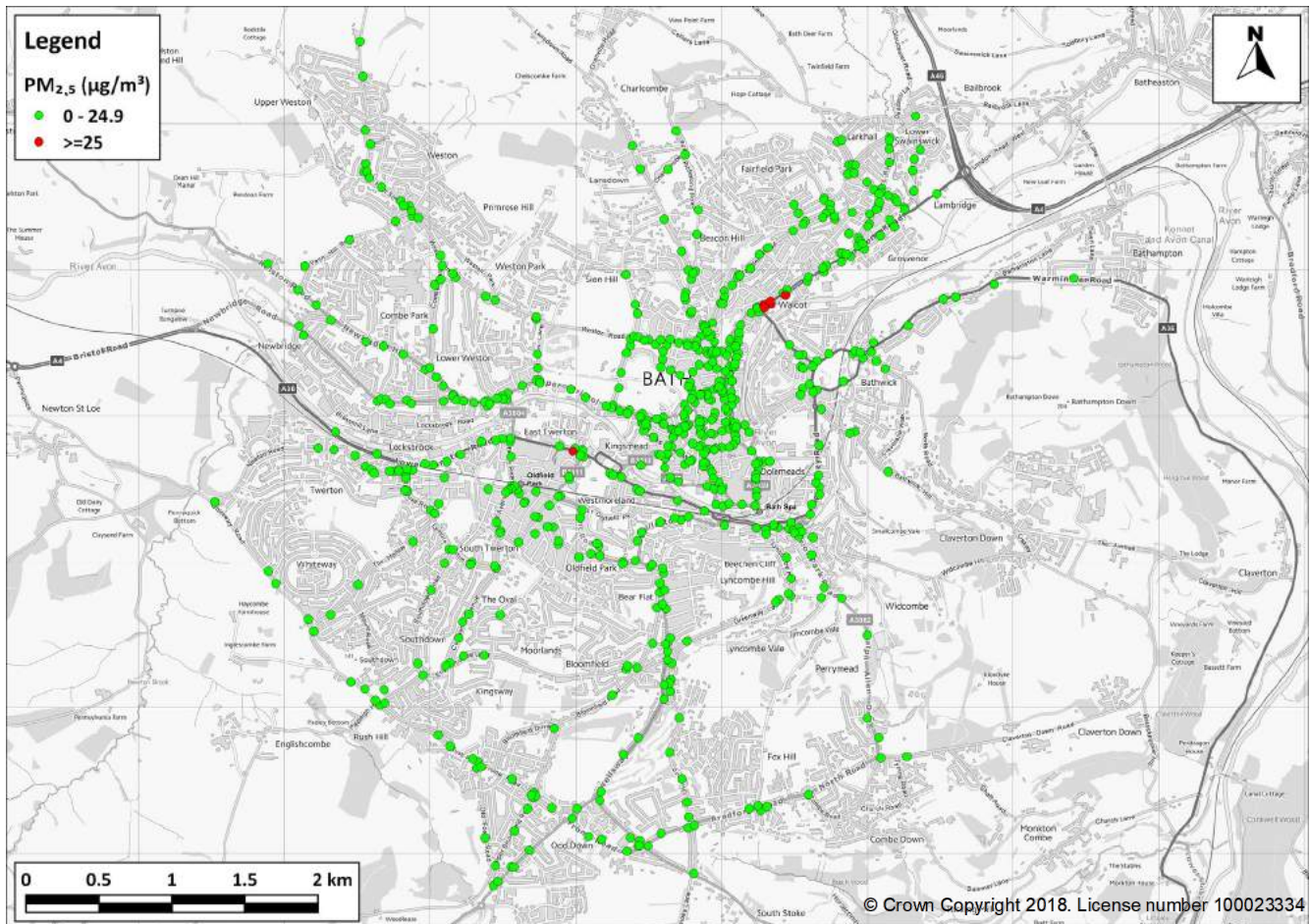
Figure 9: Predicted PM 2.5 concentrations in 2017 at receptor locations relevant to the national air quality objective (annual mean)
