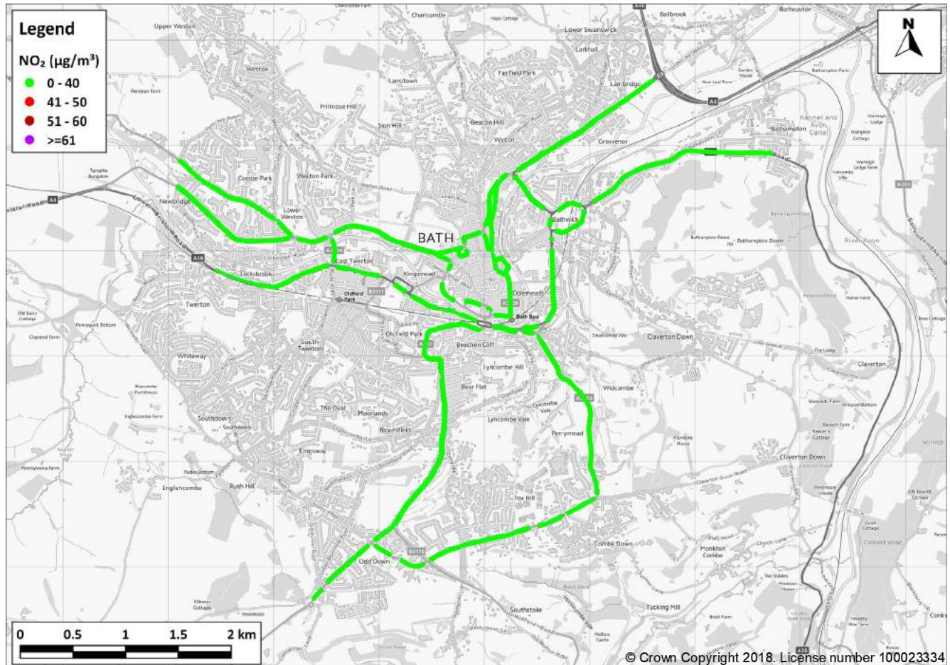
Figure 19: Predicted NO 2 concentrations in 2021 with a CAZ D (£9/£100 charge) at PCM-equivalent receptor locations (annual mean)
