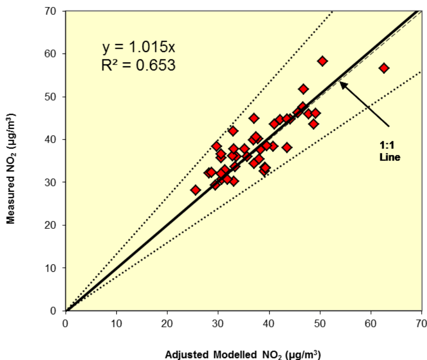
Figure 9: Comparison of Measured Total NO 2 to Final Adjusted Modelled Total NO 2 Concentrations. The dashed lines show \pm 25\% .
