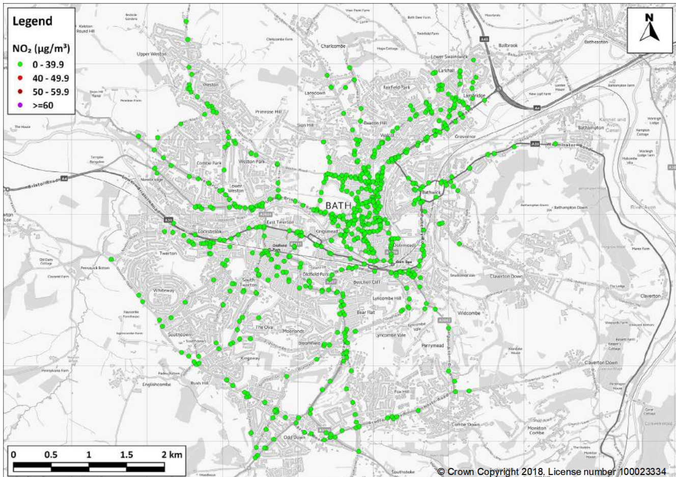
Figure 20: Predicted NO 2 concentrations in 2021 with a CAZ D (£9/£100 charge) at receptor locations relevant to the national air quality objective (annual mean)
