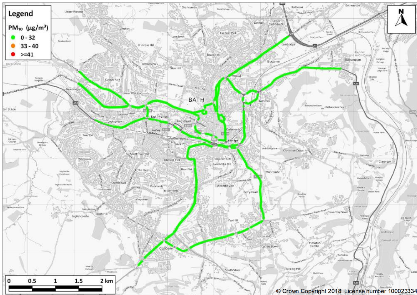
Figure 12: Predicted PM 10 concentrations in 2021 at PCM-equivalent receptor locations
