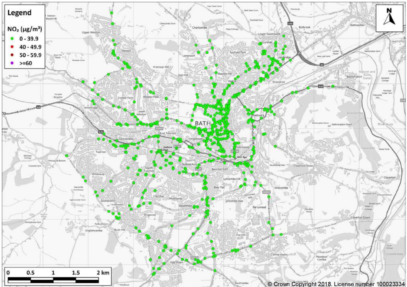
Figure 22: Predicted NO 2 concentrations in 2021 with a CAZ C (£9/£100 charge) with Traffic Management at receptor locations relevant to the national air quality objective (annual mean)
