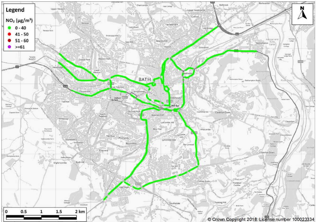
Figure 25: Predicted NO 2 concentrations in 2021 with a CAZ C (£9/£100 charge) with Traffic Management (Revised Boundary) at PCM-equivalent receptor locations (annual mean)
