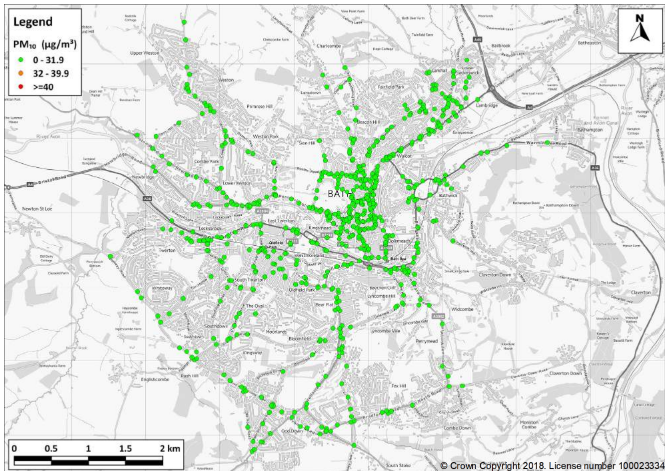
Figure 8: Predicted PM 10 concentrations in 2021 at receptor locations relevant to the national air quality objective (annual mean)
