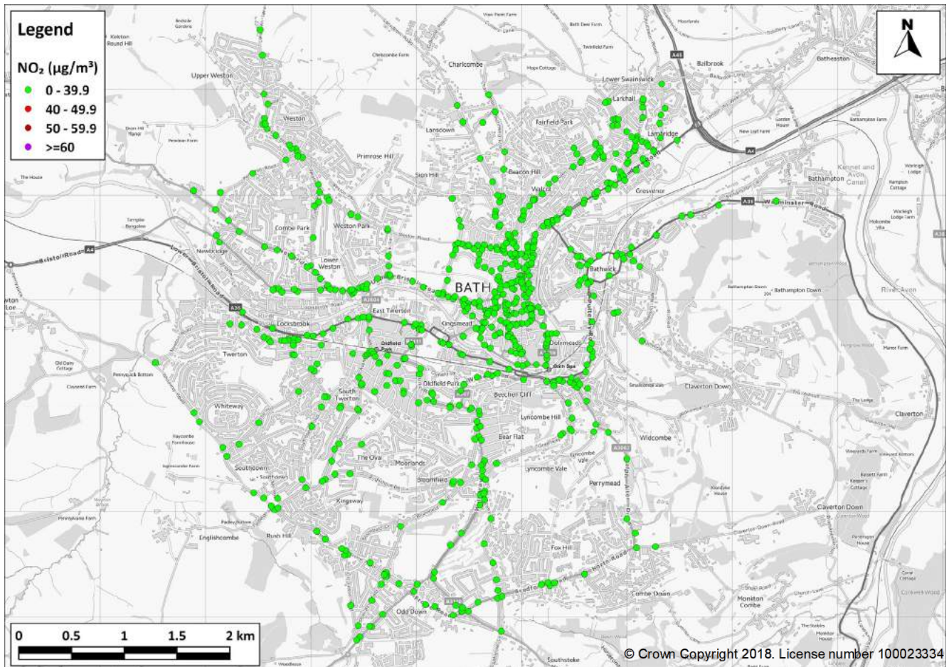
Figure 16: Predicted NO 2 concentrations in 2021 with a CAZ C (£9/£100 charge) at receptor locations relevant to the national air quality objective (annual mean)
