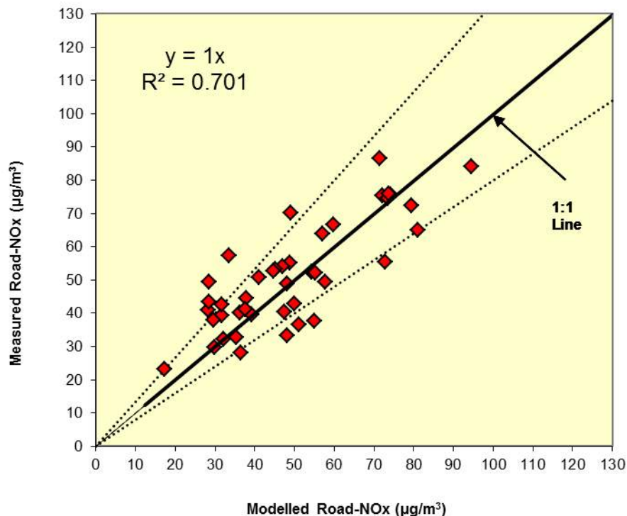
Figure 1: Comparison of Measured and Modelled Road-NO x Concentrations (following adjustments to emissions). The dashed lines show \pm 25\% .
