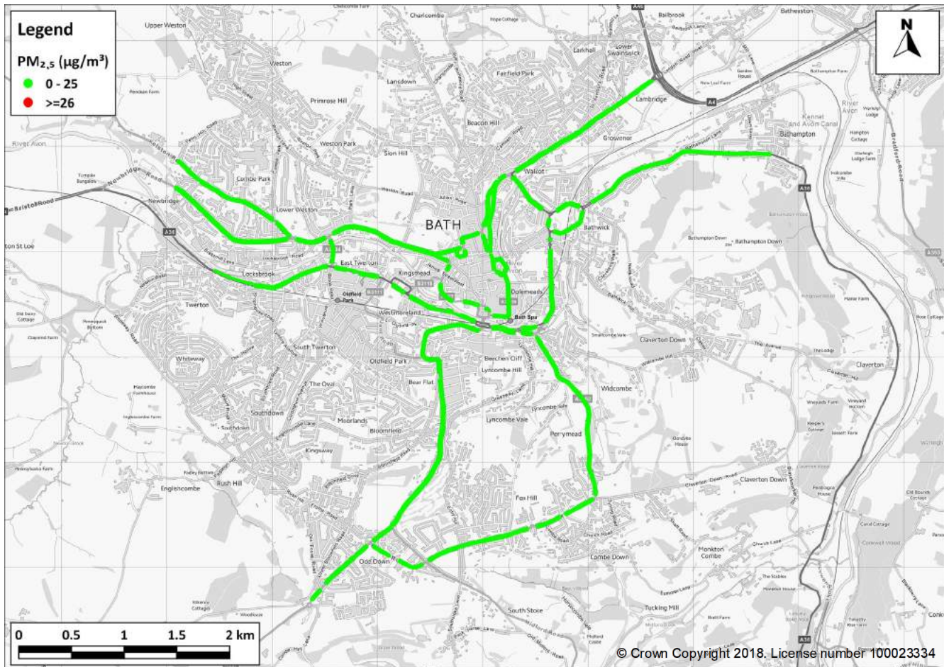
Figure 14: Predicted PM 2.5 concentrations in 2021 at PCM-equivalent receptor locations
