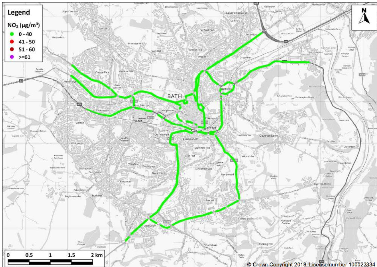
Figure 23: Predicted NO 2 concentrations in 2021 with a CAZ D (£9/£100 charge) With Traffic Management and Concessions at PCM-equivalent receptor locations (annual mean)
